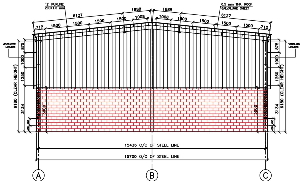
ELEVATION FOR END WALL
