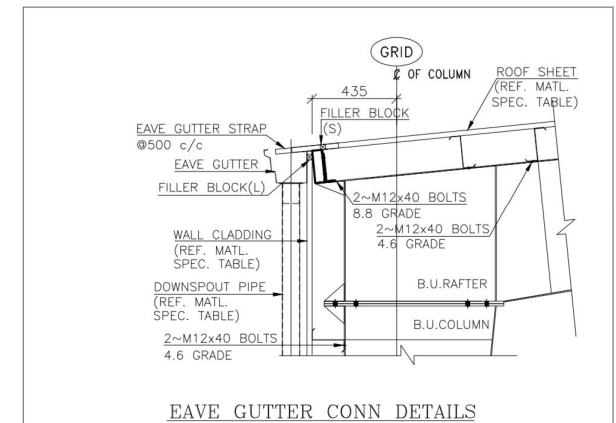
EAVE GUTTER CONN DETAILS
