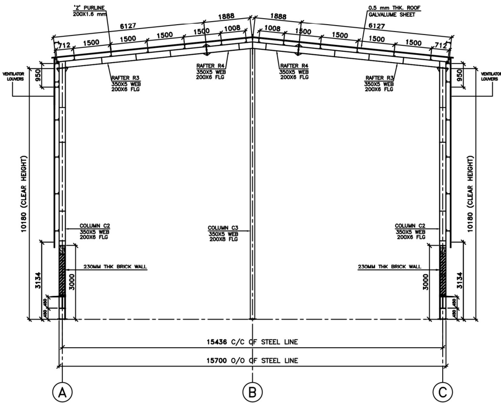
PORTAL FRAME AT GRID 1 & 3.
