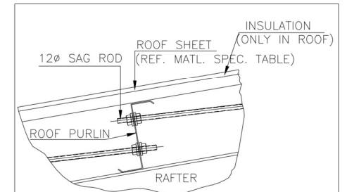
TYPICAL SAG ROD DETAIL
