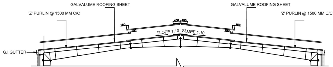
TYP. ROOF SHEETING DETAILS
