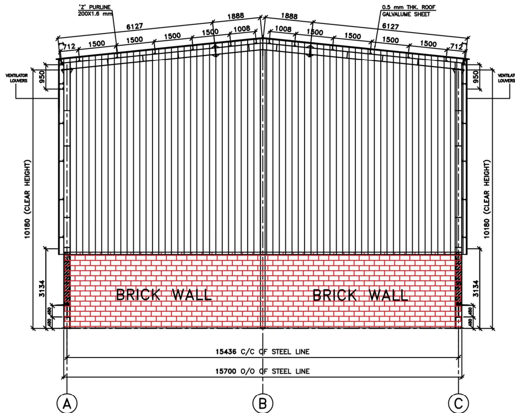
PORTAL FRAME AT GRID 1 & 3.
